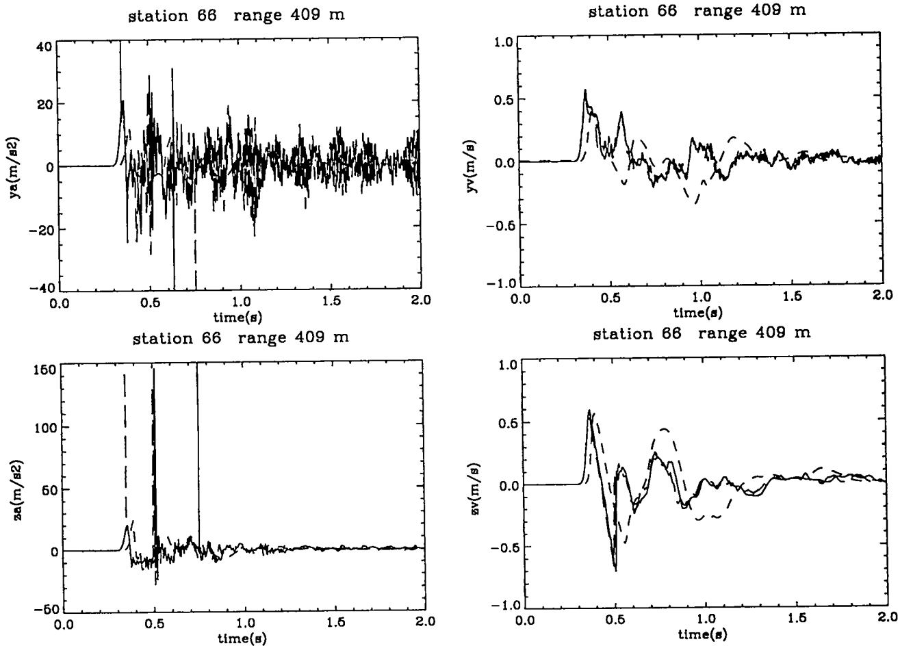
Figure 47: Experimental and computational free-surface results at 409 m. Shown are the radial acceleration ( m/s^2 ), radial velocity ( m/s ), vertical acceleration ( m/s^2 ), and vertical velocity ( m/s ) vs. time ( s ) at 409 m range from the NPE SGZ. The solid line denotes the CE simulation; the long dashed line represents the NE simulation; the short dashed line represents the NPE data collected by LLNL [33], gage H3.
