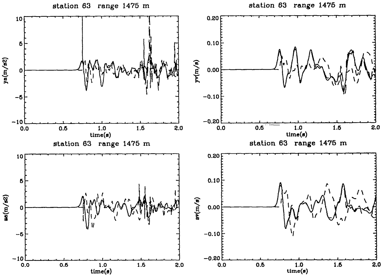
Figure 64: Experimental and computational free-surface results at 1475 m. Shown are the radial acceleration (m/s 2 ), radial velocity (m/s), vertical acceleration (m/s 2 ), and vertical velocity (m/s) vs. time (s) at 1475 m range from the NPE SGZ. The solid line denotes the CE simulation; the long dashed line represents the NE simulation; the short dashed line represents the NPE data collected by LANL [34], gage S2P.
