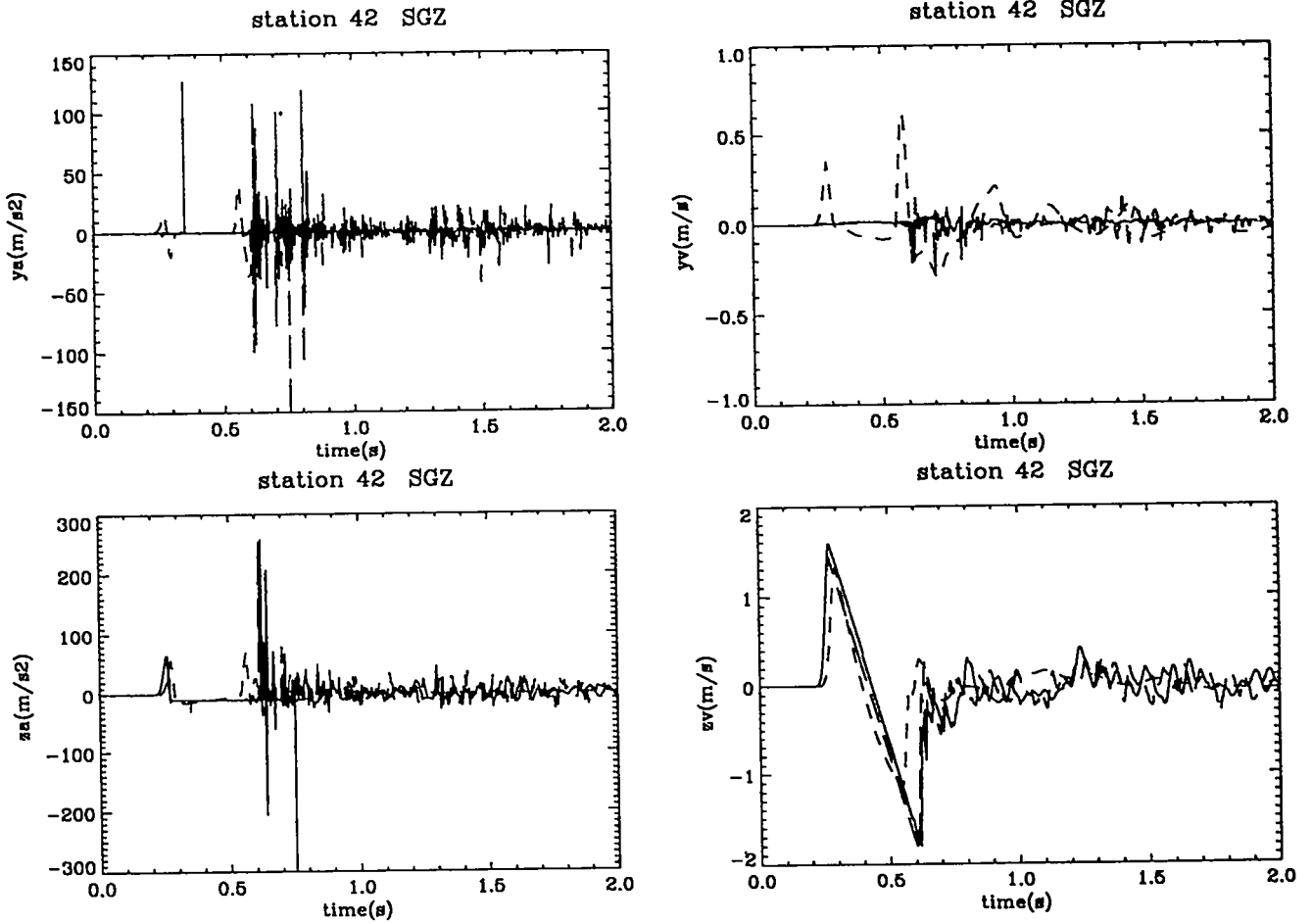
Figure 41: Experimental and computational free-surface results at SGZ. Shown are the radial acceleration ( m/s^2 ), radial velocity ( m/s ), vertical acceleration ( m/s^2 ), and vertical velocity ( m/s ) vs. time (s) at the NPE SGZ. The solid line denotes the CE simulation; the long dashed line represents the NE simulation; the short dashed line represents the NPE data collected by LLNL [33], gage GZ. The vertical velocity amplitude and dwell compare favorably between experiment and calculation. The strong signal in experimental radial velocity suggests that the true first surface arrival point may not have been at SGZ.
