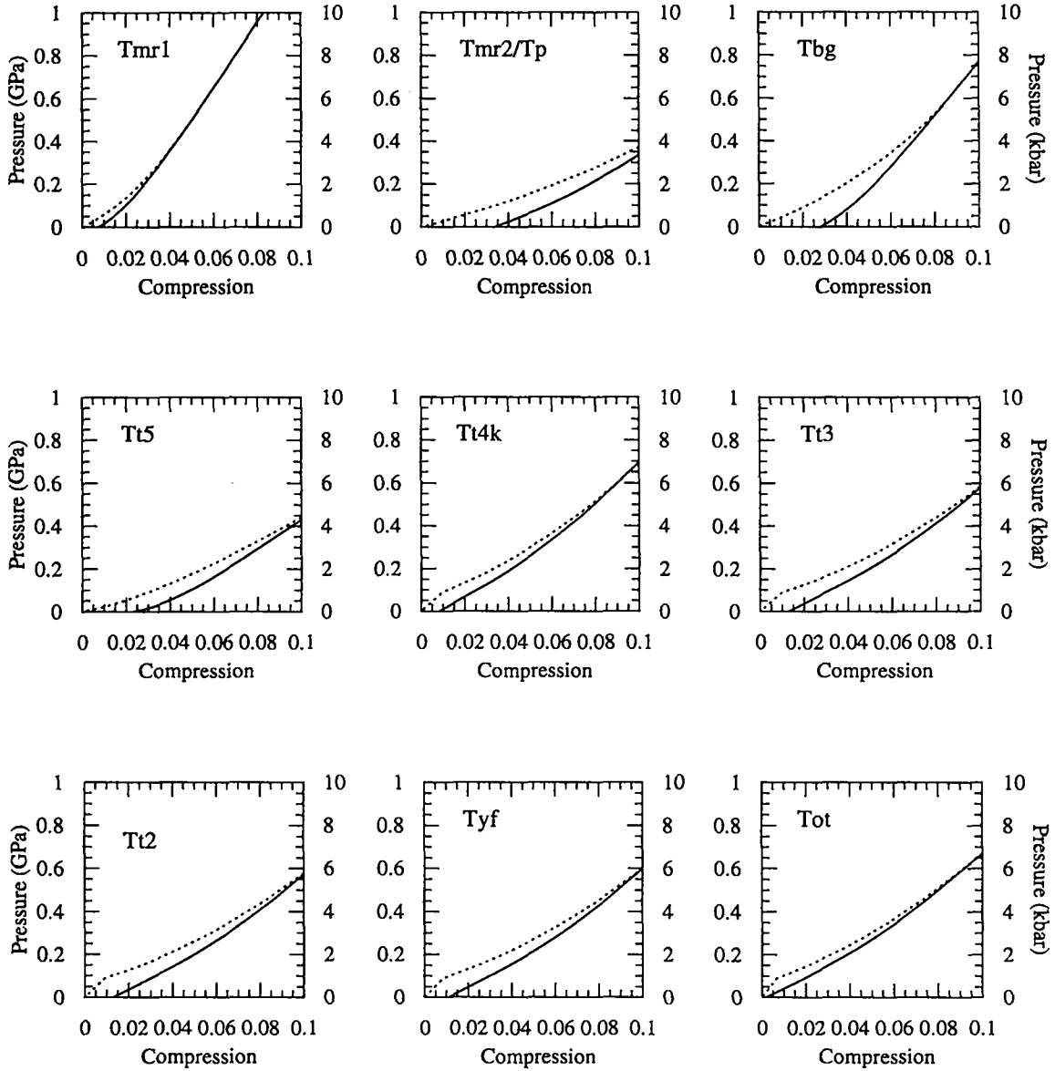
Figure 3: Pressure-volume relationship for NPE geologic materials. Shown are the pressure (GPa) vs. compression ( \mu \equiv (\rho/\rho_0) - 1 ) curves for the various geologic materials used in the two-dimensional, cylindrically symmetric NPE simulations. The upper curve in each plot depicts the crush-up response of the virgin material, while the lower curve gives the behavior of the completely crushed rock.
