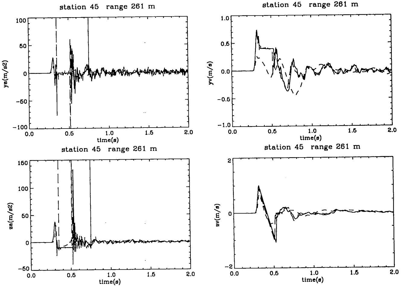
Figure 43: Experimental and computational free-surface results at 261 m. Shown are the radial acceleration (m/s 2 ), radial velocity (m/s), vertical acceleration (m/s 2 ), and vertical velocity (m/s) vs. time (s) at 261 m range from the NPE SGZ. The solid line denotes the CE simulation; the long dashed line represents the NE simulation; the short dashed line represents the NPE data collected by LLNL [33], gage E1.
