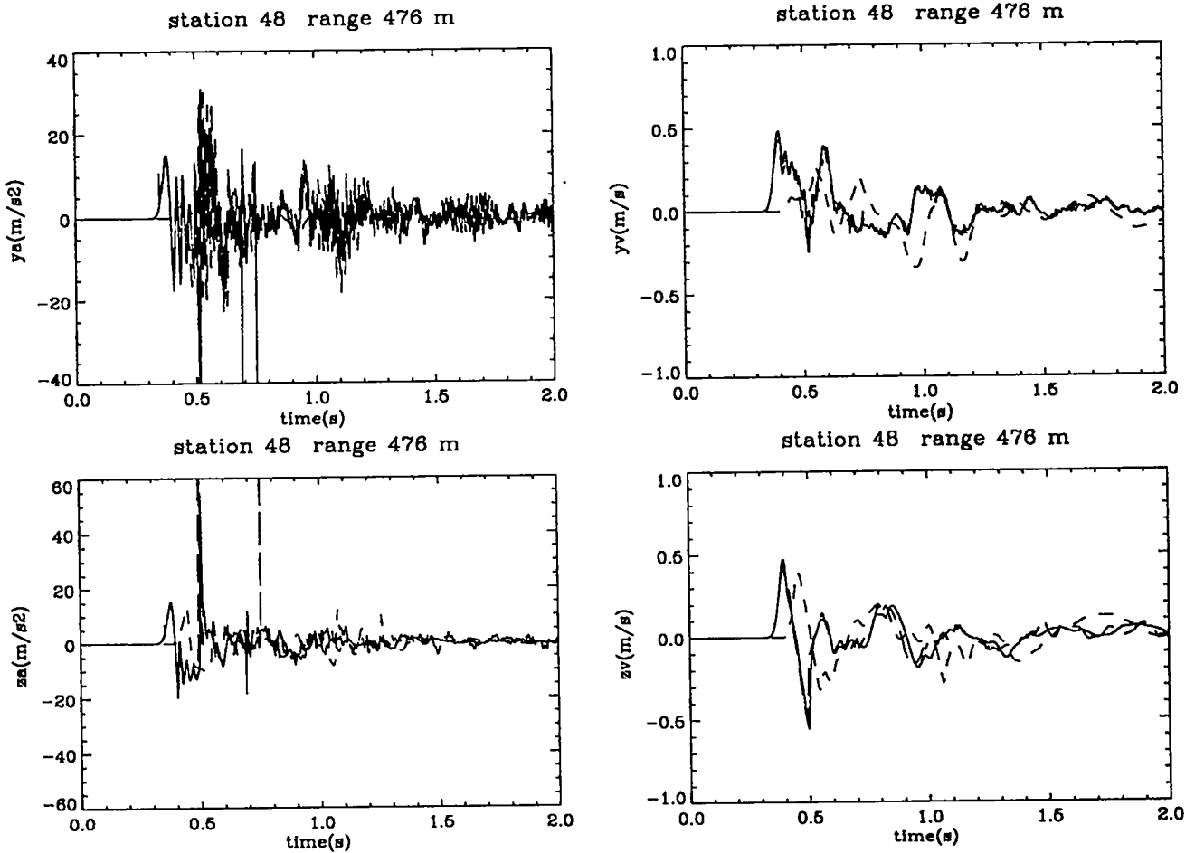
Figure 49: Experimental and computational free-surface results at 476 m. Shown are the radial acceleration (m/s 2 ), radial velocity (m/s), vertical acceleration (m/s 2 ), and vertical velocity (m/s) vs. time (s) at 476 m range from the NPE SGZ. The solid line denotes the CE simulation; the long dashed line represents the NE simulation; the short dashed line represents the NPE data collected by LANL [34], gage H9A.
