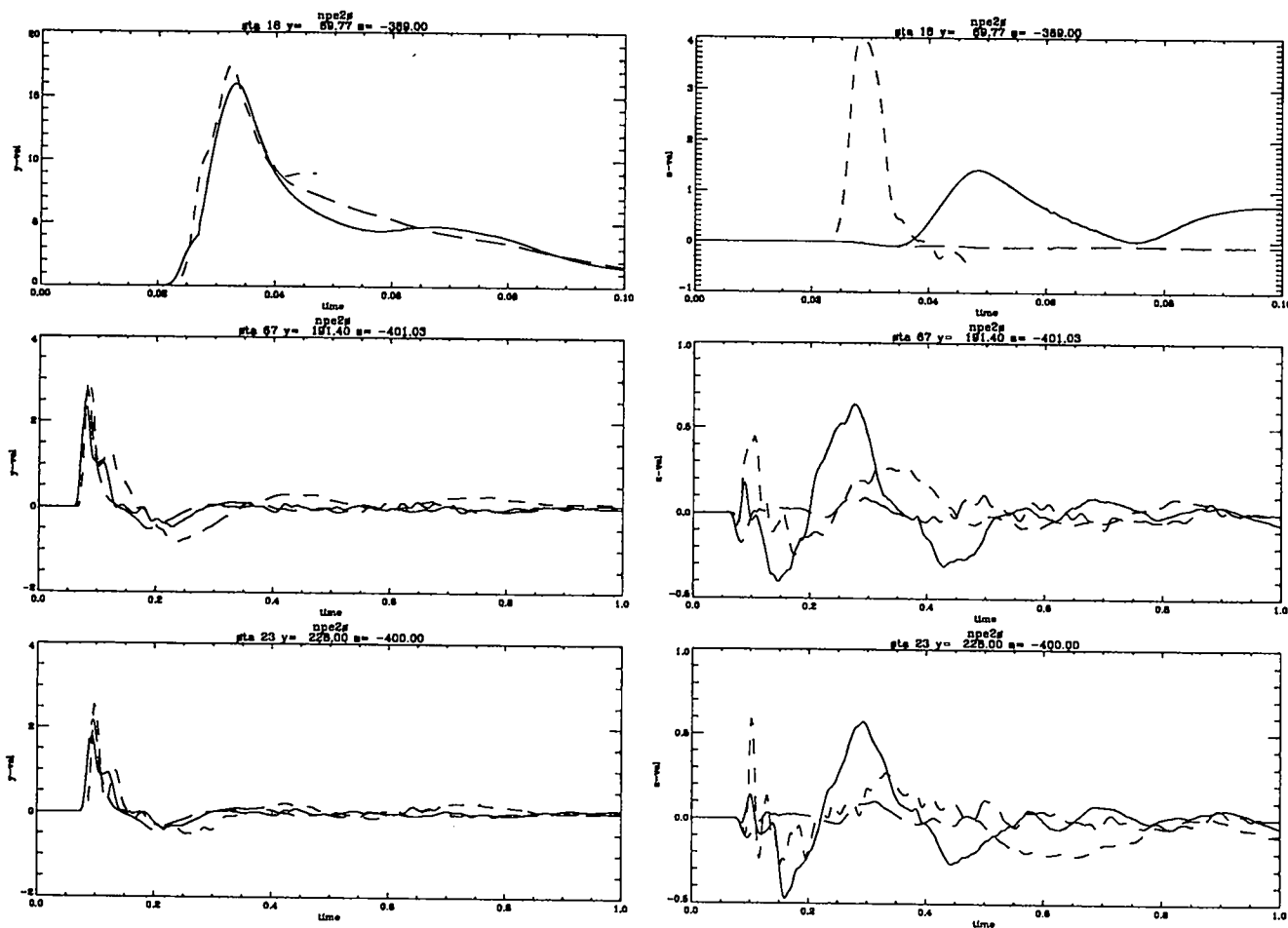
Figure 31: Near source free-field velocities: uniform and layered geologies. Shown are the radial (left) and vertical (right) velocity (m/s) vs. time (s) at shot depth for ranges of 70 m, 191 m, and 228 m from the NPE WP. The solid lines denote the layered geology CE simulations; the long dashed lines represent the uniform WP geology CE simulations; the short dashed line represents the NPE data collected by LANL P-15 [21] and SNLA [22]. The significant differences exhibited in the vertical velocity traces are presumably a manifestation of layering effects. Similarly, the post-initial-peak “plateau” in radial velocity evident in the experimental data and layered calculation at 191 m and 228 m is probably related to layering, as this structure is not present in the uniform calculation.
