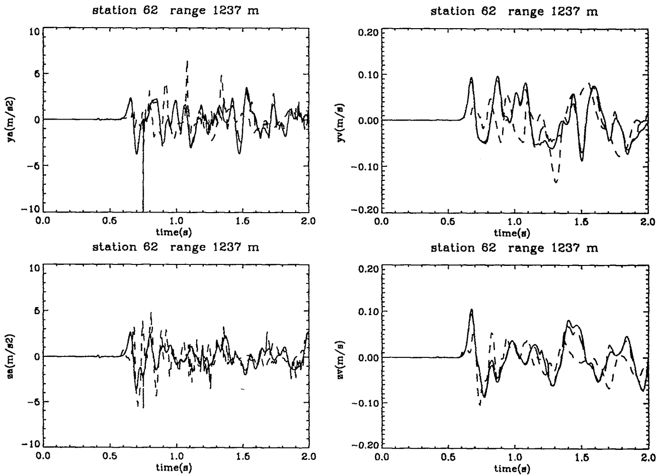
Figure 62: Experimental and computational free-surface results at 1237 m. Shown are the radial acceleration (m/s 2 ), radial velocity (m/s), vertical acceleration (m/s 2 ), and vertical velocity (m/s) vs. time (s) at 1237 m range from the NPE SGZ. The solid line denotes the CE simulation; the long dashed line represents the NE simulation; the short dashed line represents the NPE data collected by LANL [34], gage S8A.
