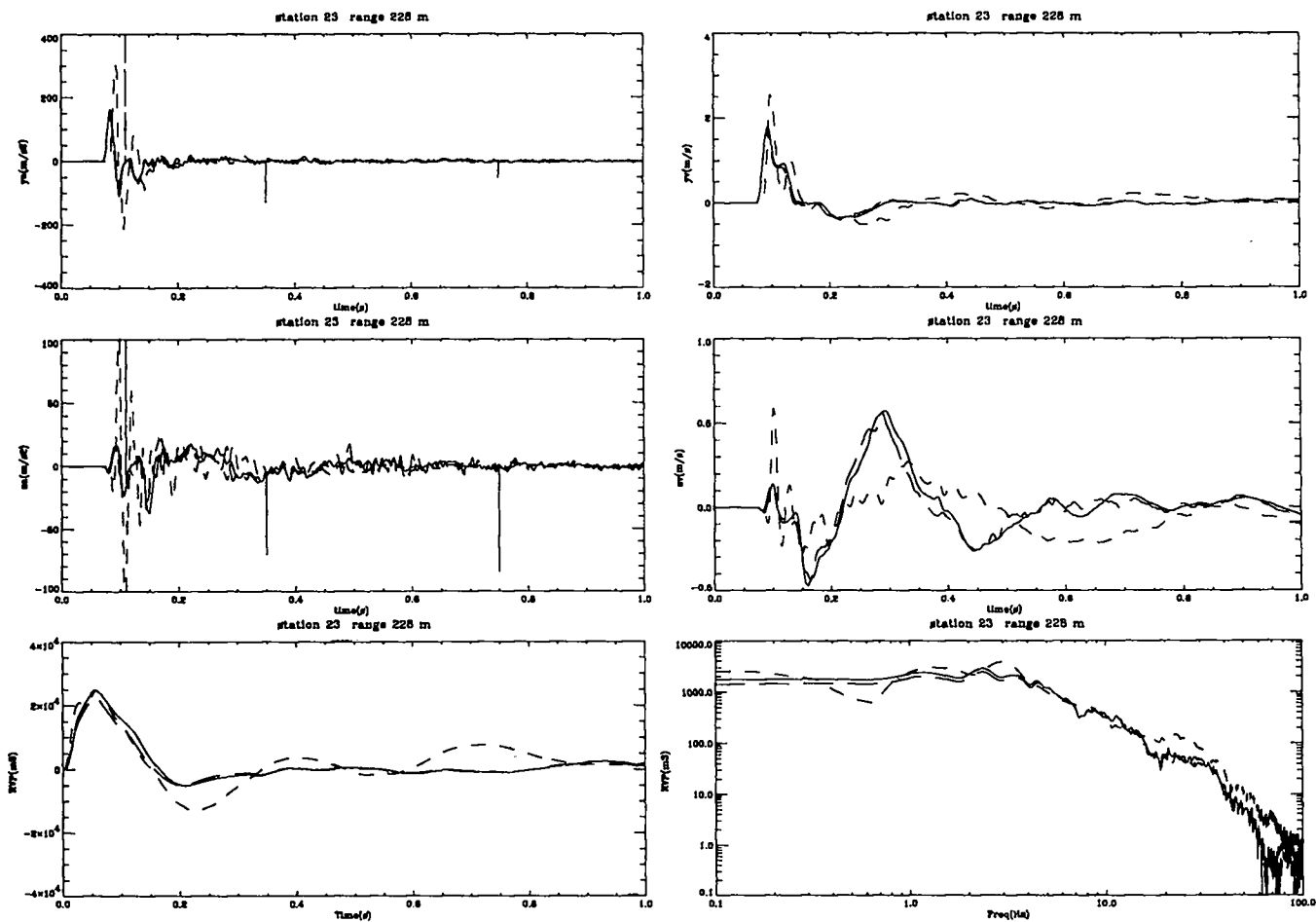
Figure 15: Experimental and computational free-field results at 228 m. Shown are the radial acceleration ( m/s^2 ), radial velocity ( m/s ), vertical acceleration ( m/s^2 ), and vertical velocity ( m/s ) vs. time (s), RVP ( m^3/s ) vs. reduced time (s), and RVP spectrum ( m^3 ) vs. frequency (Hz) at shot depth and 228 m range from the NPE WP. Only the first 1 s of the calculated results are depicted. The solid lines denote the CE simulations; the long dashed lines represent the NE simulations; the short dashed line represents the NPE data collected by LANL P-15 [21], gage TM7.
