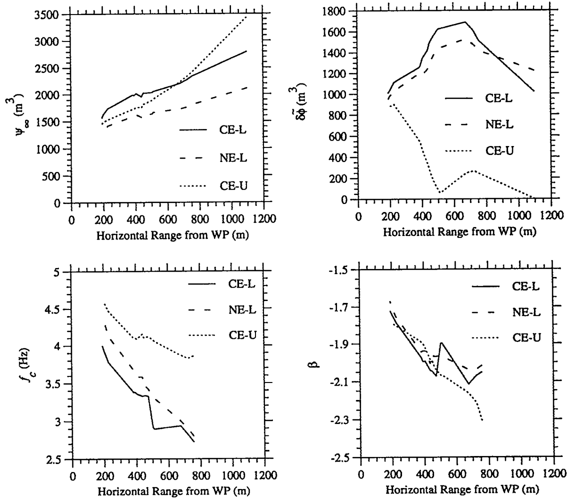
Figure 35: Computed free-field seismic source function parameters vs. range (m) at locations beyond the elastic radius. Clockwise from the upper left, these plots are of the final RDP value \psi_{\infty} (m 3 ), the RVP spectrum overshoot \delta\tilde{\phi} (m 3 ), the RVP spectrum roll-off \beta , and the RVP spectrum corner frequency f_c (Hz) for the layered CE simulation (solid line), the layered NE simulation (dashed line), and the uniform CE simulation (dotted line).
