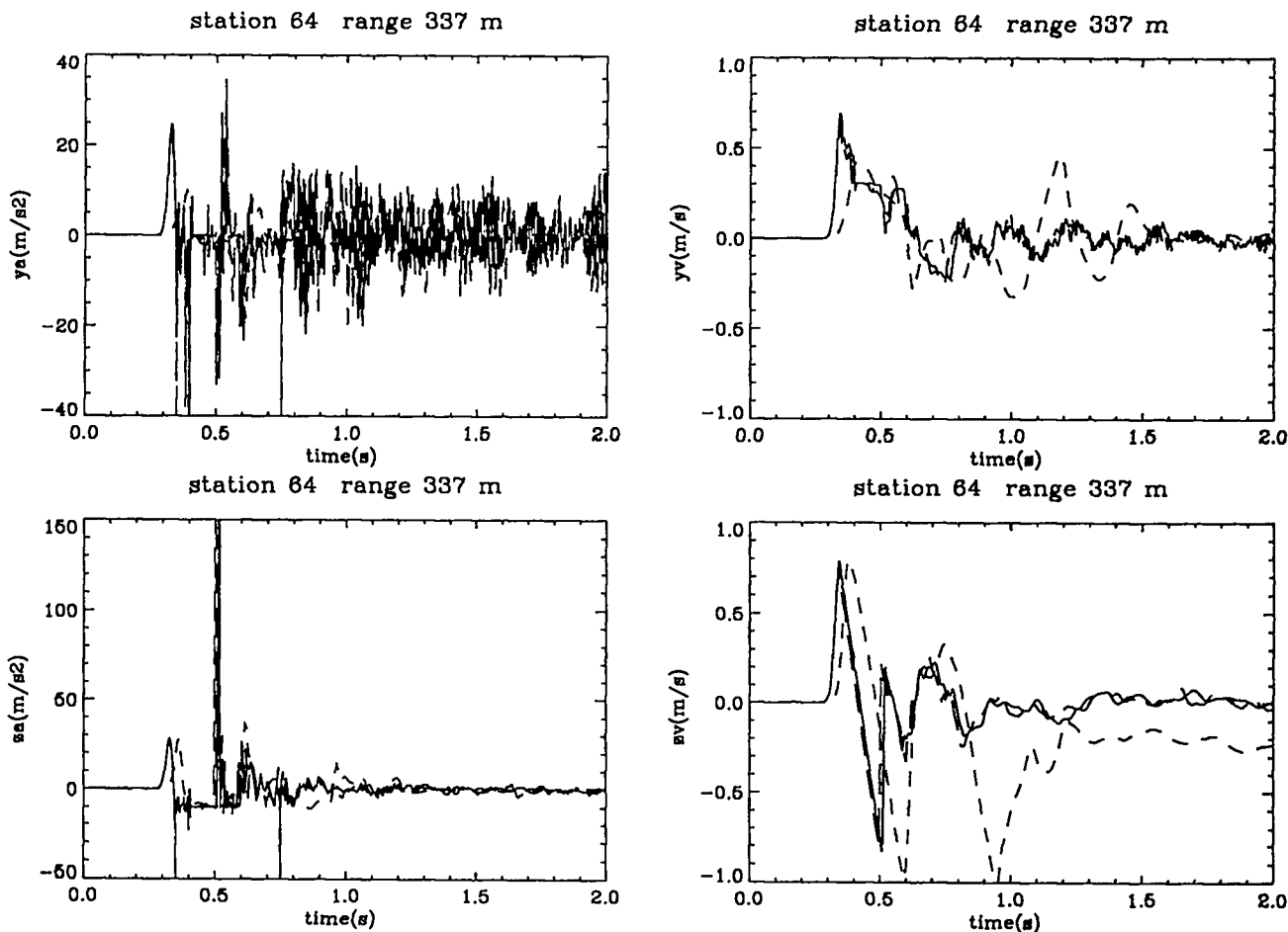
Figure 45: Experimental and computational free-surface results at 337 m. Shown are the radial acceleration (m/s 2 ), radial velocity (m/s), vertical acceleration (m/s 2 ), and vertical velocity (m/s) vs. time (s) at 337 m range from the NPE SGZ. The solid line denotes the CE simulation; the long dashed line represents the NE simulation; the short dashed line represents the NPE data collected by LLNL [33], gage H7.
