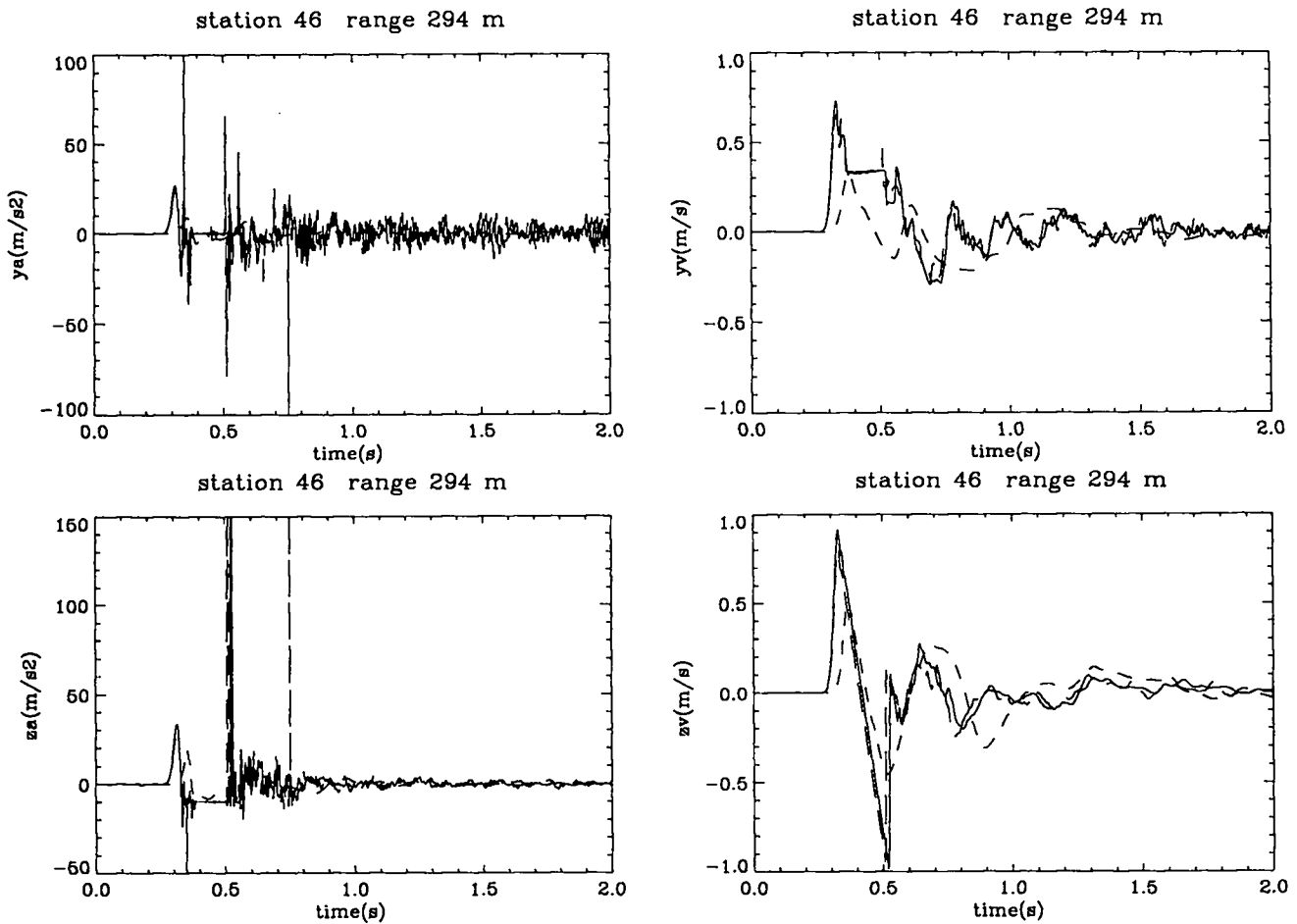
Figure 44: Experimental and computational free-surface results at 294 m. Shown are the radial acceleration ( m/s^2 ), radial velocity ( m/s ), vertical acceleration ( m/s^2 ), and vertical velocity ( m/s ) vs. time (s) at 294 m range from the NPE SGZ. The solid line denotes the CE simulation; the long dashed line represents the NE simulation; the short dashed line represents the NPE data collected by LLNL [33], gage Q4.
