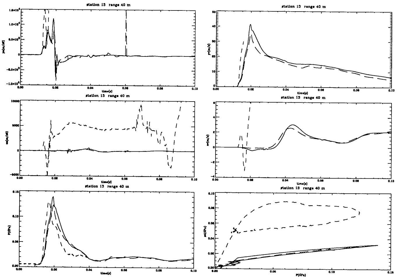
Figure 8: Experimental and computational free-field results at 40 m. Shown are the radial acceleration ( m/s^2 ), radial velocity ( m/s ), tangential acceleration ( m/s^2 ), tangential velocity ( m/s ), and pressure (GPa) vs. time (s), and stress difference (GPa) (i.e., absolute value of radial stress minus tangential stress) vs. pressure (GPa) at shot depth and 40 m range from the NPE WP. Only the first 100 ms of the calculated results are depicted. The solid lines denote the CE simulations; the long dashed lines represent the NE simulations; the short dashed line represents the NPE data collected by SNLA [18], gages 3YR, 3YT, 3AR, 3AT (see Table 4).
