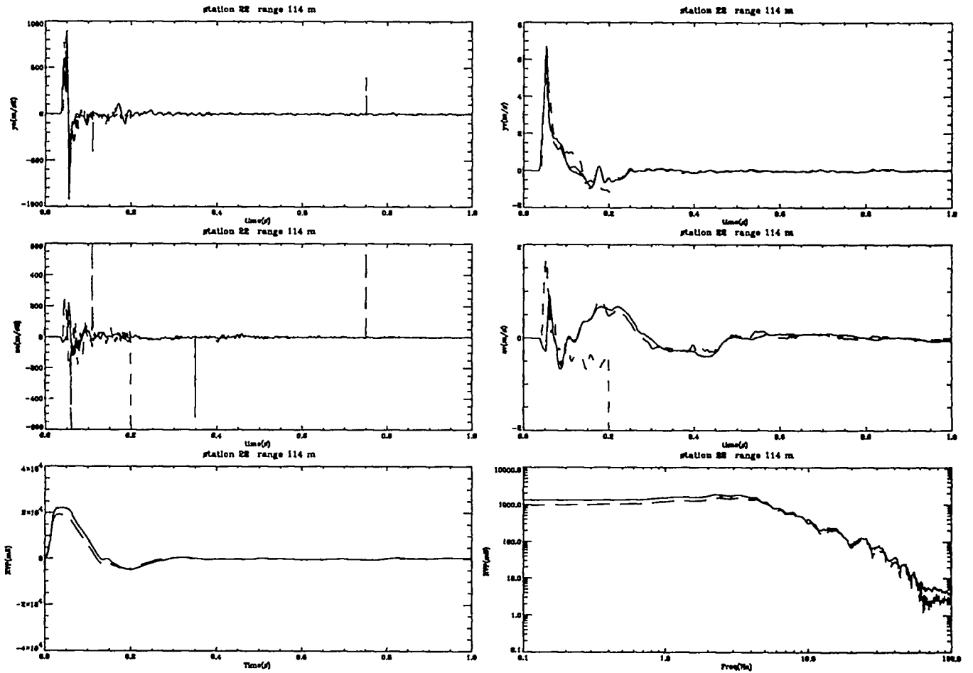
Figure 12: Experimental and computational free-field results at 114 m. Shown are the radial acceleration ( m/s^2 ), radial velocity ( m/s ), vertical acceleration ( m/s^2 ), and vertical velocity ( m/s ) vs. time (s), RVP ( m^3/s ) vs. reduced time (s), and RVP spectrum ( m^3 ) vs. frequency (Hz) at shot depth and 114 m range from the NPE WP. Only the first 1 s of the calculated results are depicted. The solid lines denote the CE simulations; the long dashed lines represent the NE simulations; the short dashed line represents the NPE data collected by LANL P-15 [21], gage TM34. There was insufficient gage data (only \sim 0.2 s) at this location to compute the RVP and RVP spectrum.
