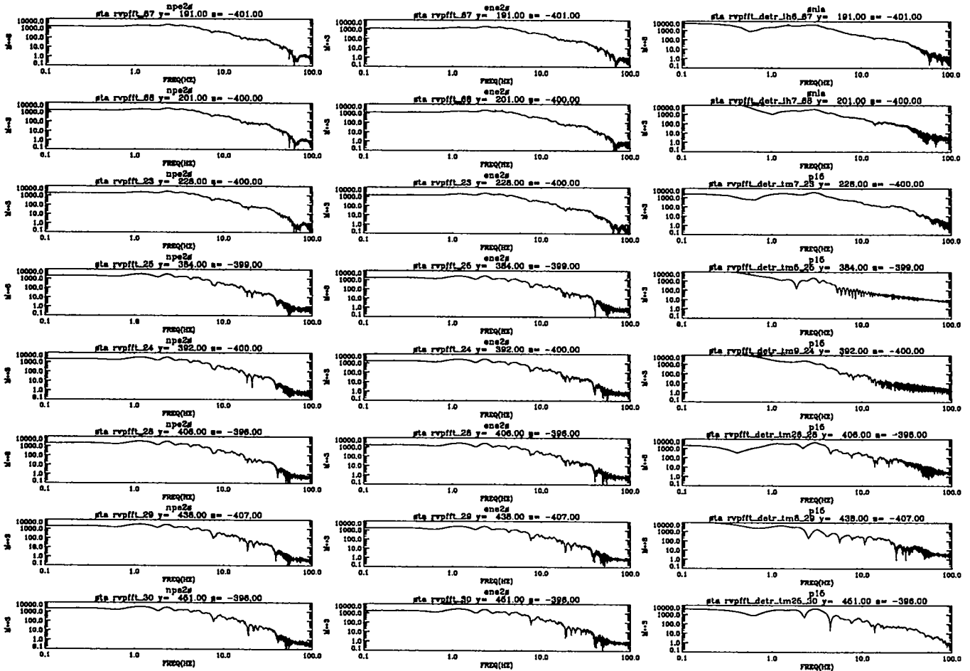
Figure 33: Near source free-field RVP spectra. The computed reduced velocity potential spectra ( \text{m}^3 ) are plotted against frequency (Hz) at near source free-field locations beyond the elastic radius. The left column contains the CE simulation results; the middle column contains the NE simulation results; the right column contains the NPE data [21, 22] results.
