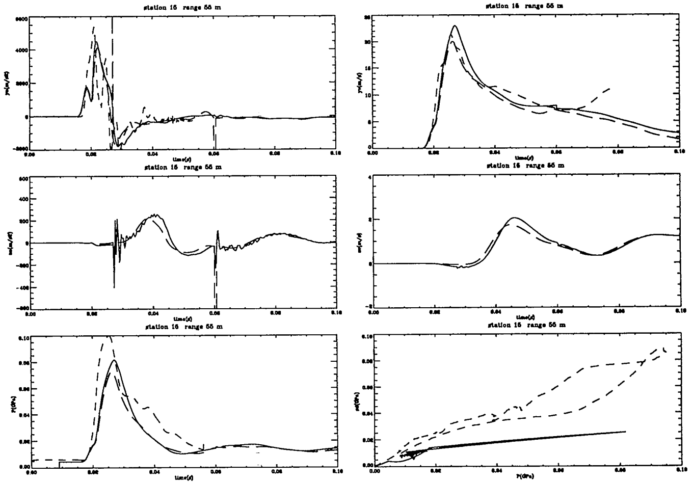
Figure 9: Experimental and computational free-field results at 55 m. Shown are the radial acceleration ( m/s^2 ), radial velocity ( m/s ), tangential acceleration ( m/s^2 ), tangential velocity ( m/s ), and pressure (GPa) vs. time (s), and stress difference (GPa) (i.e., absolute value of radial stress minus tangential stress) vs. pressure (GPa) at shot depth and 55 m range from the NPE WP. Only the first 100 ms of the calculated results are depicted. The solid lines denote the CE simulations; the long dashed lines represent the NE simulations; the short dashed line represents the NPE data collected by SNLA [18], gage 4YR, 4YT, 4AR (see Table 4). There are no z-acceleration or z-velocity data at this station.
