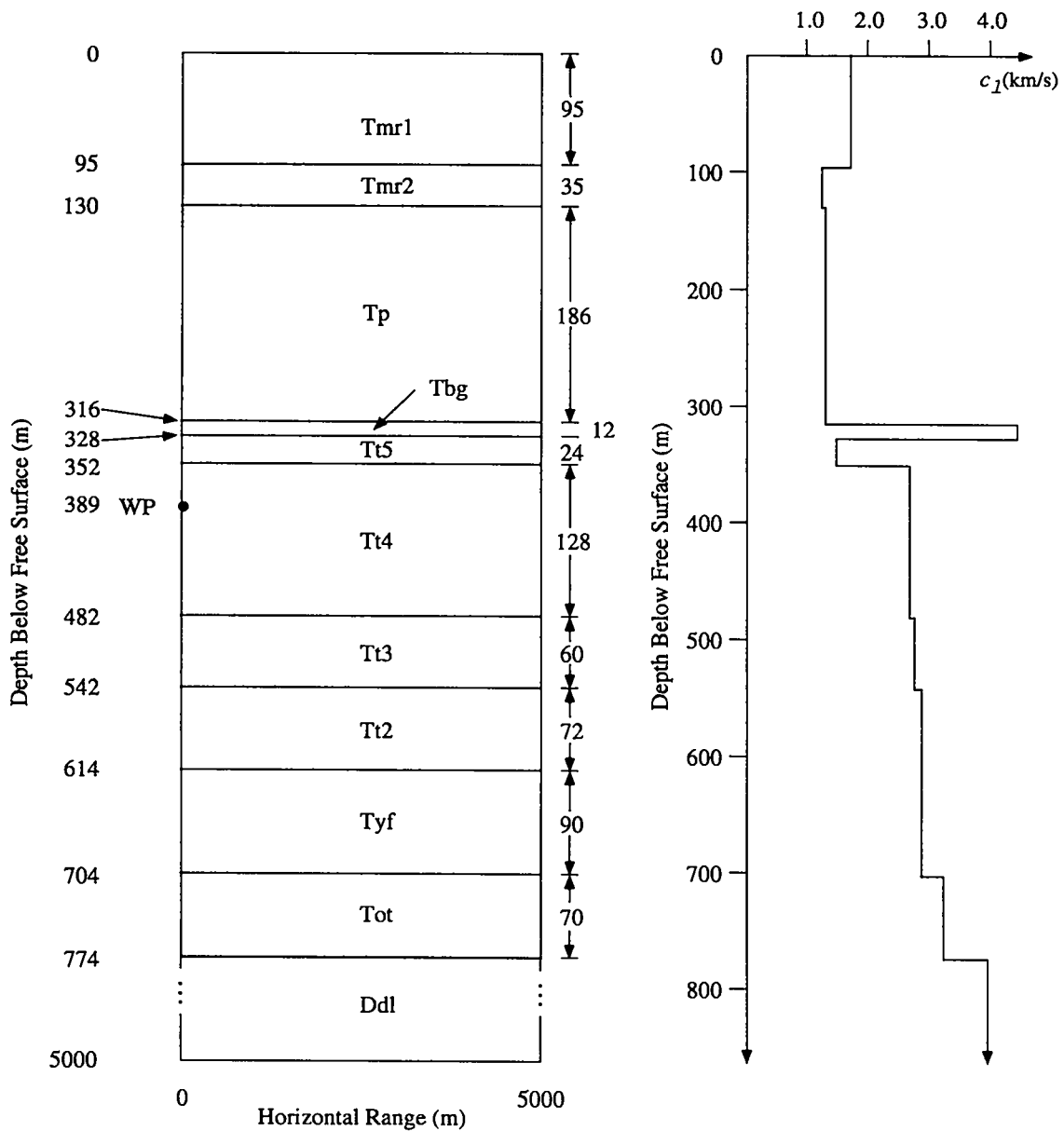
Figure 2: Layering model for the NPE simulations. Depicted are the stratigraphic model (left) and velocity profile (right) used in the two-dimensional, cylindrically symmetric NPE simulations. The material properties ascribed to the media in the various layers are catalogued in Tables 1 and 2. In this figure, distances are in m and velocities are in km/s. There are notable impedance mismatches around the thin Tbg layer, and at the zeolitization boundary between the Tt4 and Tt5 units.
