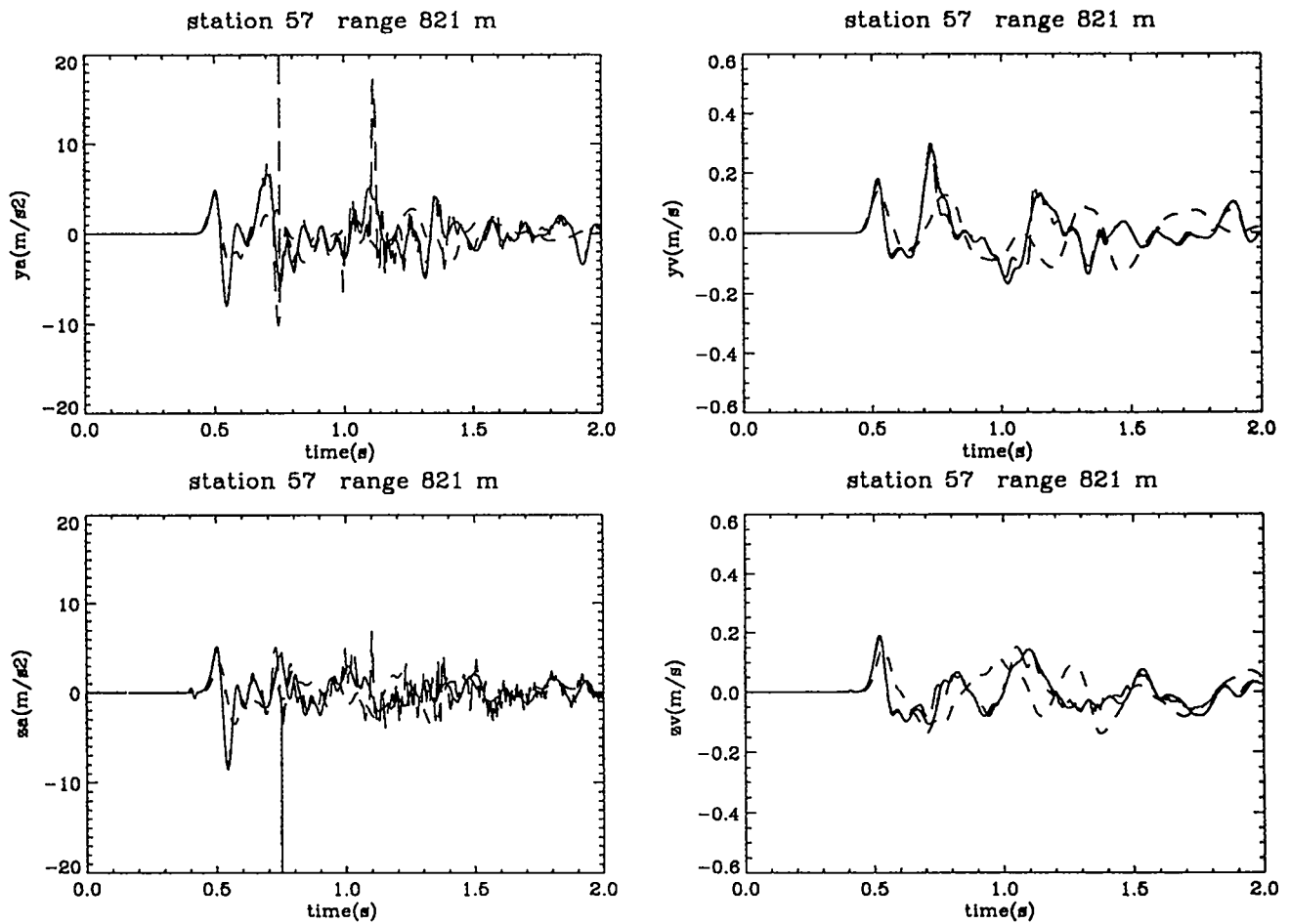
Figure 58: Experimental and computational free-surface results at 821 m. Shown are the radial acceleration (m/s 2 ), radial velocity (m/s), vertical acceleration (m/s 2 ), and vertical velocity (m/s) vs. time (s) at 821 m range from the NPE SGZ. The solid line denotes the CE simulation; the long dashed line represents the NE simulation; the short dashed line represents the NPE data collected by LLNL [33], gage Q3.
