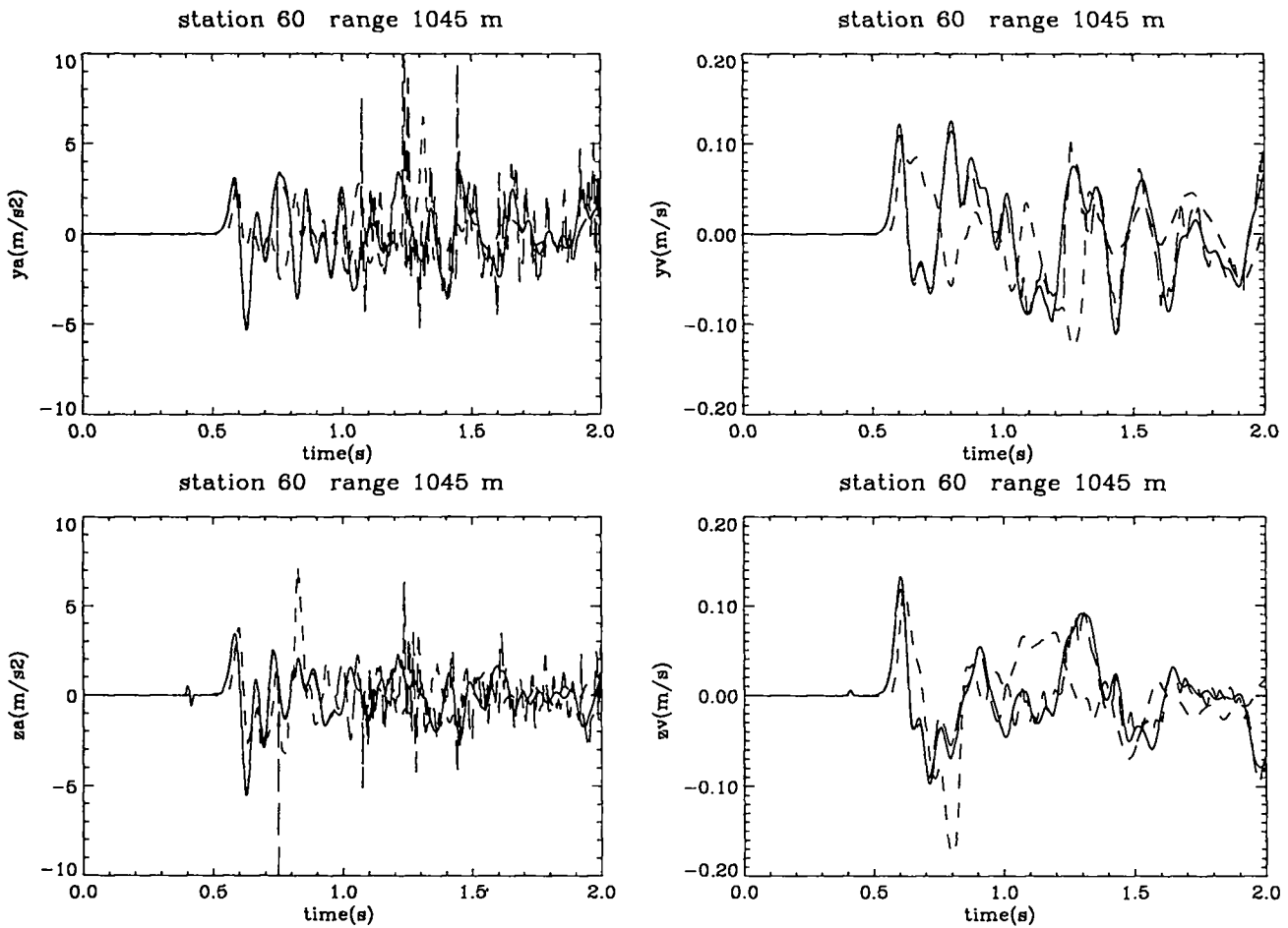
Figure 61: Experimental and computational free-surface results at 1045 m. Shown are the radial acceleration (m/s 2 ), radial velocity (m/s), vertical acceleration (m/s 2 ), and vertical velocity (m/s) vs. time (s) at 1045 m range from the NPE SGZ. The solid line denotes the CE simulation; the long dashed line represents the NE simulation; the short dashed line represents the NPE data collected by LANL [34], gage S4P.
