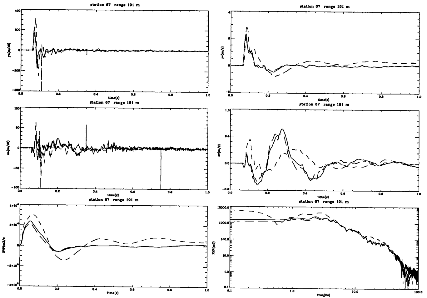
Figure 13: Experimental and computational free-field results at 191 m. Shown are the radial acceleration (m/s 2 ), radial velocity (m/s), vertical acceleration (m/s 2 ), and vertical velocity (m/s) vs. time (s), RVP (m 3 /s) vs. reduced time (s), and RVP spectrum (m 3 ) vs. frequency (Hz) at shot depth and 191 m range from the NPE WP. Only the first 1 s of the calculated results are depicted. The solid lines denote the CE simulations; the long dashed lines represent the NE simulations; the short dashed line represents the NPE data collected by H. D. Garbin of SNLA [22], gage IH6.
