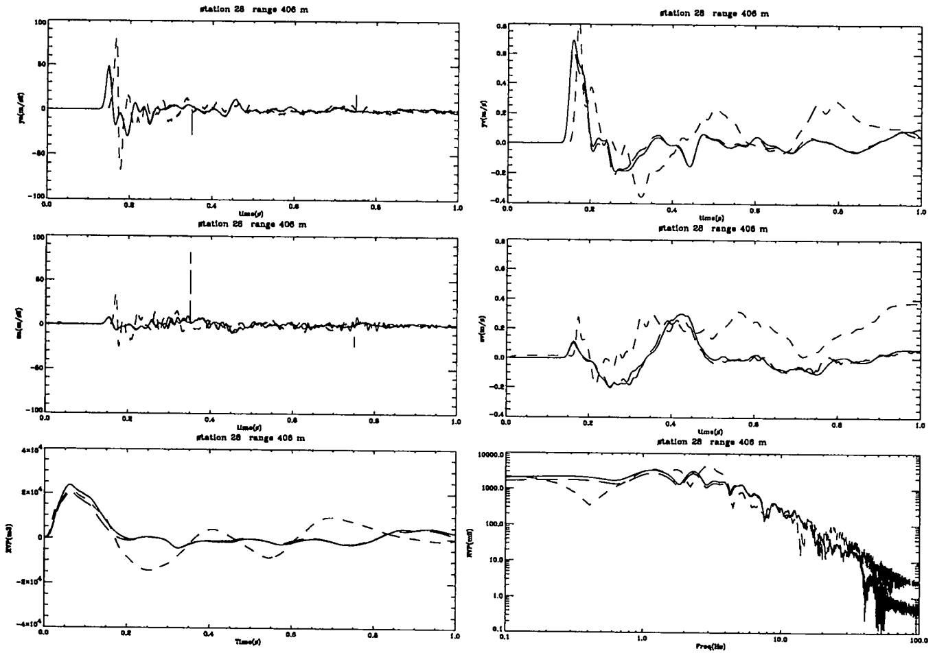
Figure 18: Experimental and computational free-field results at 406 m. Shown are the radial acceleration (m/s 2 ), radial velocity (m/s), vertical acceleration (m/s 2 ), and vertical velocity (m/s) vs. time (s), RVP (m 3 /s) vs. reduced time (s), and RVP spectrum (m 3 ) vs. frequency (Hz) at shot depth and 406 m range from the NPE WP. Only the first 1 s of the calculated results are depicted. The solid lines denote the CE simulations; the long dashed lines represent the NE simulations; the short dashed line represents the NPE data collected by LANL P-15 [21], gage TM26.
