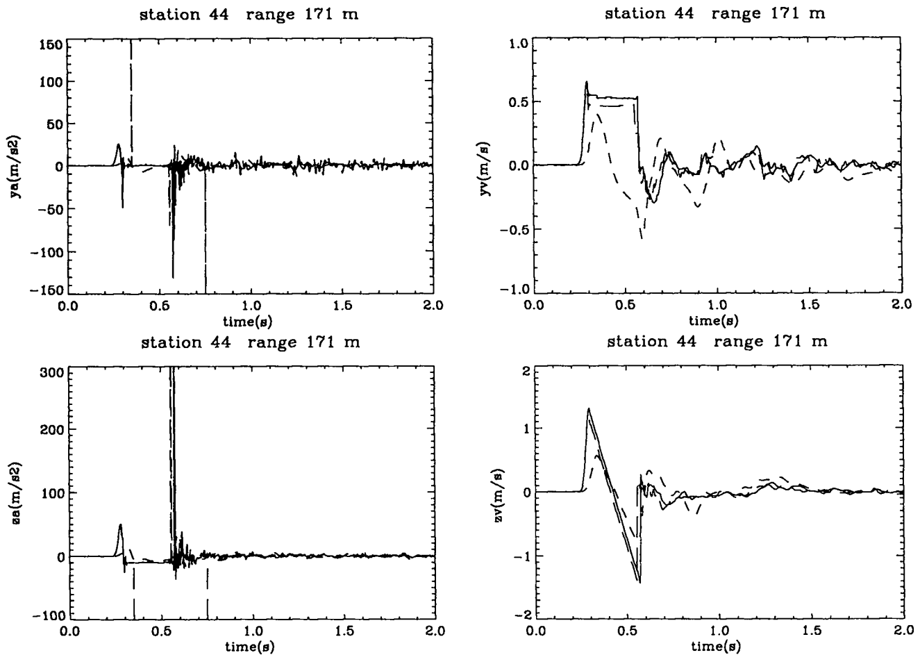
Figure 42: Experimental and computational free-surface results at 171 m. Shown are the radial acceleration ( m/s^2 ), radial velocity ( m/s ), vertical acceleration ( m/s^2 ), and vertical velocity ( m/s ) vs. time (s) at 171 m range from the NPE SGZ. The solid line denotes the CE simulation; the long dashed line represents the NE simulation; the short dashed line represents the NPE data collected by LLNL [33], gage E4.
