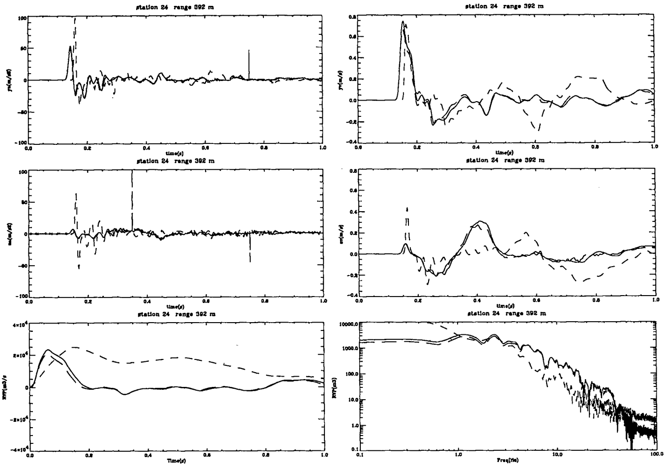
Figure 17: Experimental and computational free-field results at 392 m. Shown are the radial acceleration ( m/s^2 ), radial velocity ( m/s ), vertical acceleration ( m/s^2 ), and vertical velocity ( m/s ) vs. time (s), RVP ( m^3/s ) vs. reduced time (s), and RVP spectrum ( m^3 ) vs. frequency (Hz) at shot depth and 392 m range from the NPE WP. Only the first 1 s of the calculated results are depicted. The solid lines denote the CE simulations; the long dashed lines represent the NE simulations; the short dashed line represents the NPE data collected by LANL P-15 [21], gage TM9.
