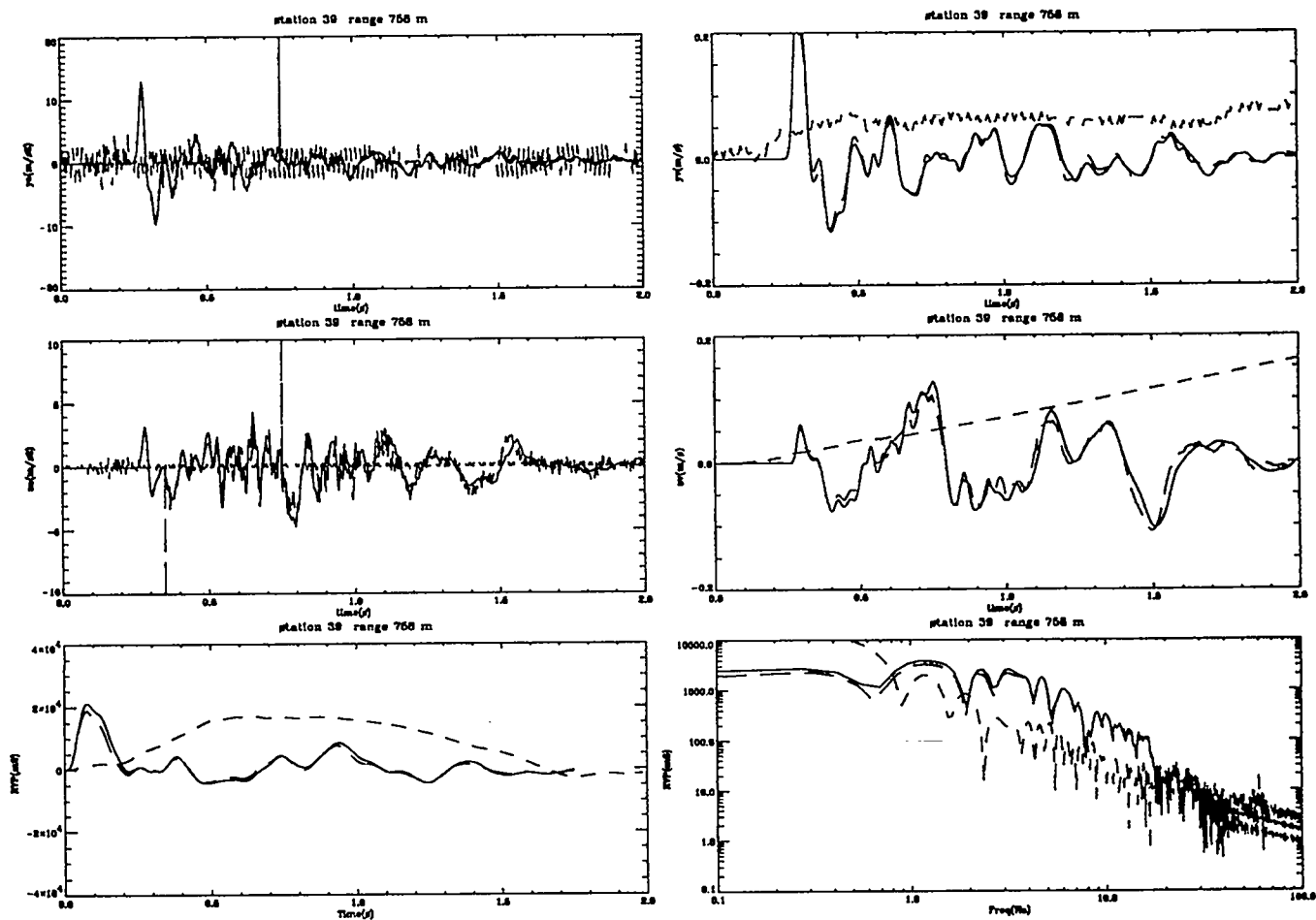
Figure 27: Experimental and computational free-field results at 758 m. Shown are the radial acceleration ( m/s^2 ), radial velocity ( m/s ), vertical acceleration ( m/s^2 ), and vertical velocity ( m/s ) vs. time (s), RVP ( m^3/s ) vs. reduced time (s), and RVP spectrum ( m^3 ) vs. frequency (Hz) at shot depth and 758 m range from the NPE WP. The solid lines denote the CE simulations; the long dashed lines represent the NE simulations; the short dashed line represents the NPE data collected by LANL P-15 [21], gage TM11. Although the data at this station appear irreparably damaged, we include them for completeness.
