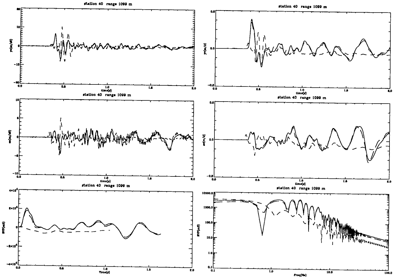
Figure 28: Experimental and computational free-field results at 1099 m. Shown are the radial acceleration ( m/s^2 ), radial velocity ( m/s ), vertical acceleration ( m/s^2 ), and vertical velocity ( m/s ) vs. time (s), RVP ( m^3/s ) vs. reduced time (s), and RVP spectrum ( m^3 ) vs. frequency (Hz) at shot depth and 1099 m range from the NPE WP. The solid lines denote the CE simulations; the long dashed lines represent the NE simulations; the short dashed line represents the NPE data collected by LANL P-15 [21], gage TM15.
