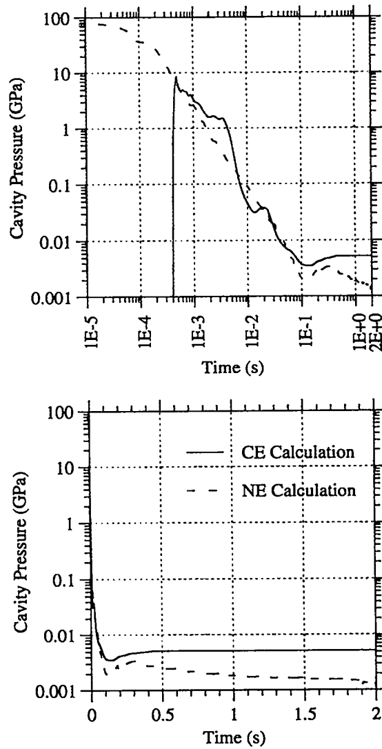
Figure 38: Cavity pressure (GPa) vs. time (s) at a point initially located 1.5 m from the cavity centerline. The upper graph, on log-log scales, demonstrates the early-time differences in cavity pressure between the chemical and nuclear source, while the lower graph, containing the same data on semilog scales, shows the late-time differences.
