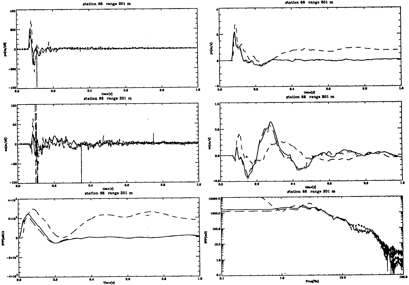
Figure 14: Experimental and computational free-field results at 201 m. Shown are the radial acceleration ( m/s^2 ), radial velocity ( m/s ), vertical acceleration ( m/s^2 ), and vertical velocity ( m/s ) vs. time (s), RVP ( m^3/s ) vs. reduced time (s), and RVP spectrum ( m^3 ) vs. frequency (Hz) at shot depth and 201 m range from the NPE WP. Only the first 1 s of the calculated results are depicted. The solid lines denote the CE simulations; the long dashed lines represent the NE simulations; the short dashed line represents the NPE data collected by H. D. Garbin of SNLA [22], gage IH7.
