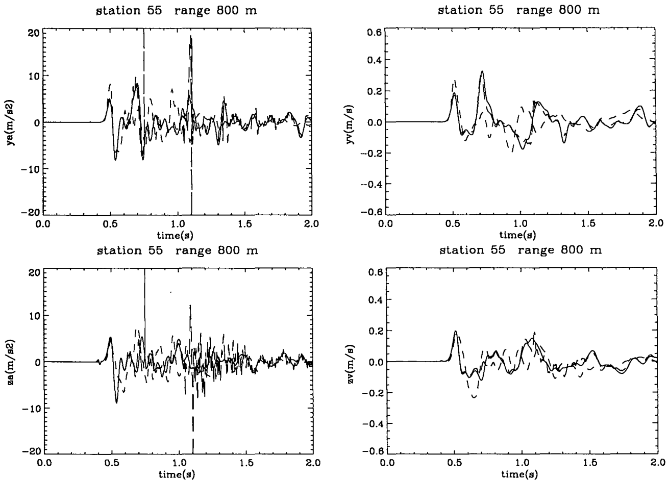
Figure 57: Experimental and computational free-surface results at 800 m. Shown are the radial acceleration (m/s 2 ), radial velocity (m/s), vertical acceleration (m/s 2 ), and vertical velocity (m/s) vs. time (s) at 800 m range from the NPE SGZ. The solid line denotes the CE simulation; the long dashed line represents the NE simulation; the short dashed line represents the NPE data collected by LANL [34], gage S10A.
