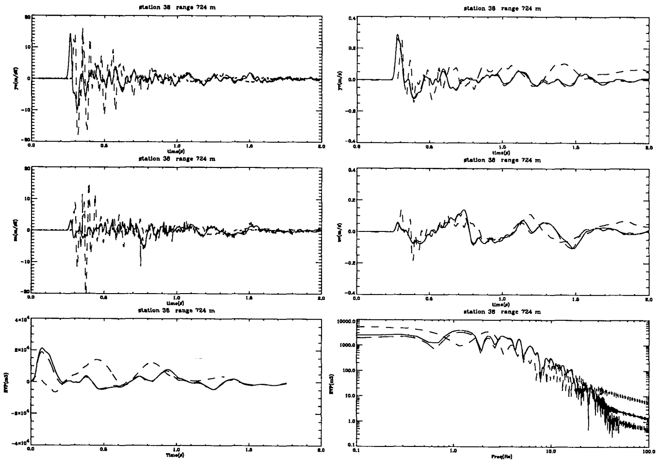
Figure 26: Experimental and computational free-field results at 724 m. Shown are the radial acceleration (m/s 2 ), radial velocity (m/s), vertical acceleration (m/s 2 ), and vertical velocity (m/s) vs. time (s), RVP (m 3 /s) vs. reduced time (s), and RVP spectrum (m 3 ) vs. frequency (Hz) at shot depth and 724 m range from the NPE WP. The solid lines denote the CE simulations; the long dashed lines represent the NE simulations; the short dashed line represents the NPE data collected by LANL P-15 [21], gage TM12.
