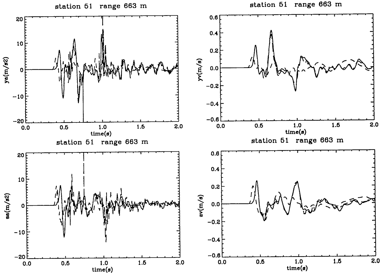
Figure 52: Experimental and computational free-surface results at 663 m. Shown are the radial acceleration (m/s 2 ), radial velocity (m/s), vertical acceleration (m/s 2 ), and vertical velocity (m/s) vs. time (s) at 663 m range from the NPE SGZ. The solid line denotes the CE simulation; the long dashed line represents the NE simulation; the short dashed line represents the NPE data collected by LANL [34], gage S6A.
