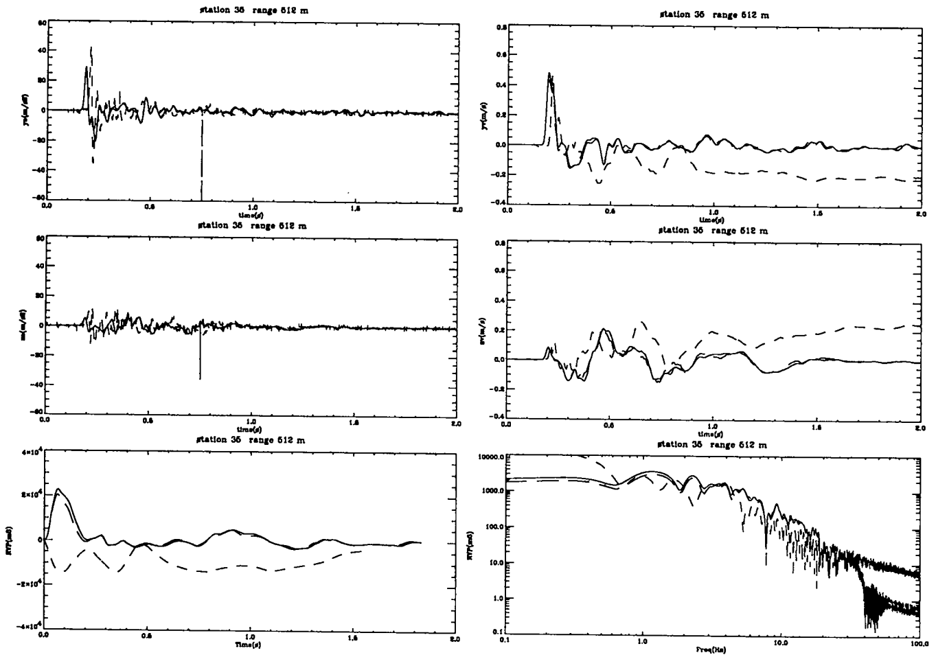
Figure 24: Experimental and computational free-field results at 512 m. Shown are the radial acceleration ( m/s^2 ), radial velocity ( m/s ), vertical acceleration ( m/s^2 ), and vertical velocity ( m/s ) vs. time (s), RVP ( m^3/s ) vs. reduced time (s), and RVP spectrum ( m^3 ) vs. frequency (Hz) at shot depth and 512 m range from the NPE WP. The solid lines denote the CE simulations; the long dashed lines represent the NE simulations; the short dashed line represents the NPE data collected by LANL P-15 [21], gage TM1.
