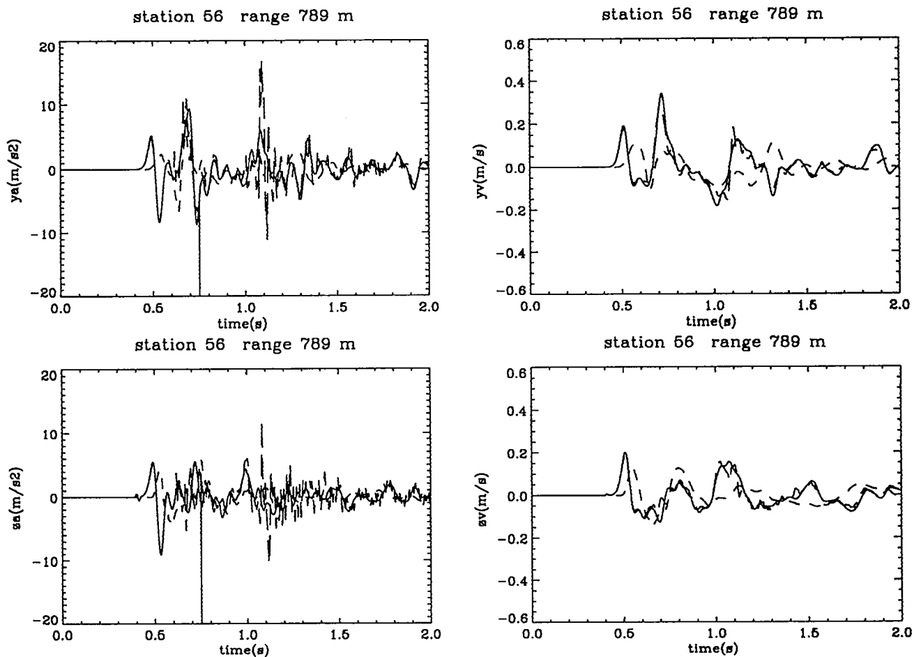
Figure 56: Experimental and computational free-surface results at 789 m. Shown are the radial acceleration (m/s 2 ), radial velocity (m/s), vertical acceleration (m/s 2 ), and vertical velocity (m/s) vs. time (s) at 789 m range from the NPE SGZ. The solid line denotes the CE simulation; the long dashed line represents the NE simulation; the short dashed line represents the NPE data collected by LANL [34], gage S6P.
