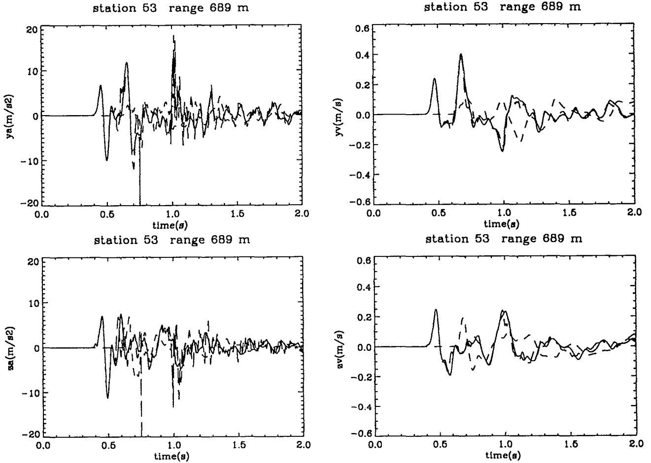
Figure 54: Experimental and computational free-surface results at 689 m. Shown are the radial acceleration (m/s 2 ), radial velocity (m/s), vertical acceleration (m/s 2 ), and vertical velocity (m/s) vs. time (s) at 689 m range from the NPE SGZ. The solid line denotes the CE simulation; the long dashed line represents the NE simulation; the short dashed line represents the NPE data collected by LANL [34], gage S10P.
