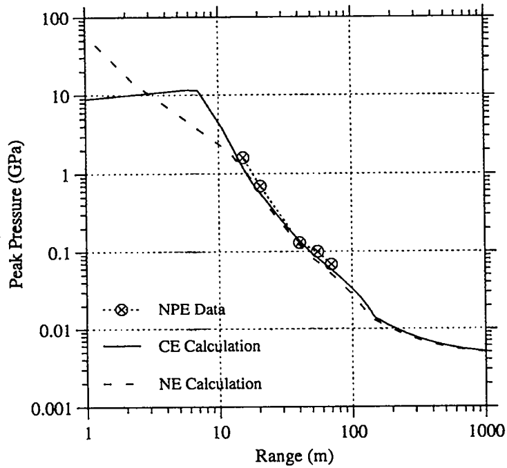
Figure 37: Peak WP-level pressure (GPa) vs. range (m) in the plane of the working point. The solid line denotes the CE simulations; the dashed line represents the NE simulations; the dotted line connects values ( \otimes ) inferred from NPE data collected by SNLA [18]. The data at the two closest ranges are peak radial stresses, which should be approximately equal to the peak pressures at these ranges [19] (i.e., assuming \sigma_{rr} \approx \sigma_{zz} \approx \sigma_{\theta\theta} ). This plot clearly illustrates one aspect of the near-source difference between chemical and nuclear sources.
