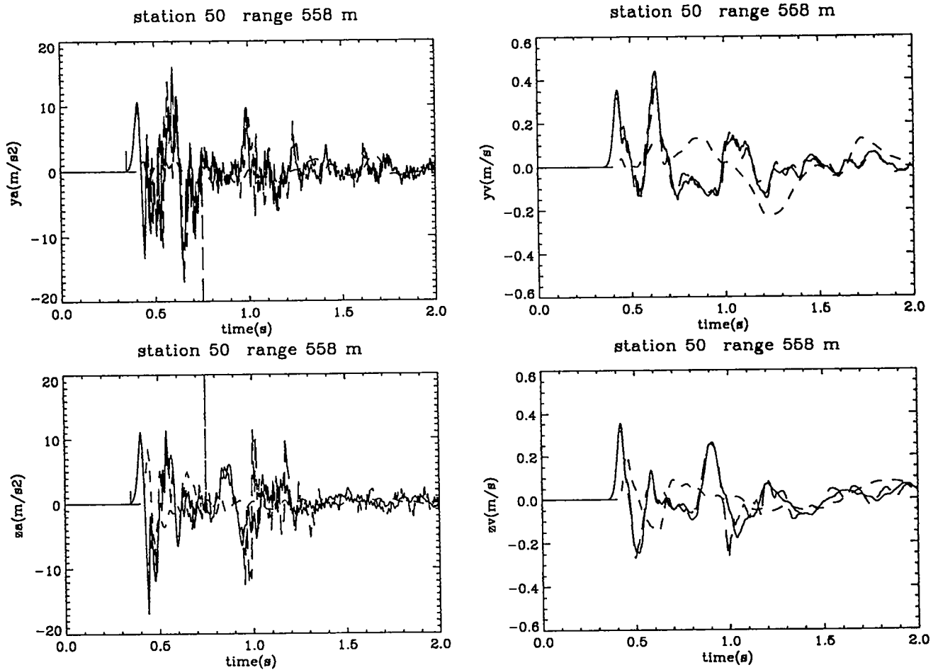
Figure 51: Experimental and computational free-surface results at 558 m. Shown are the radial acceleration (m/s 2 ), radial velocity (m/s), vertical acceleration (m/s 2 ), and vertical velocity (m/s) vs. time (s) at 558 m range from the NPE SGZ. The solid line denotes the CE simulation; the long dashed line represents the NE simulation; the short dashed line represents the NPE data collected by LLNL [33], gage E10.
