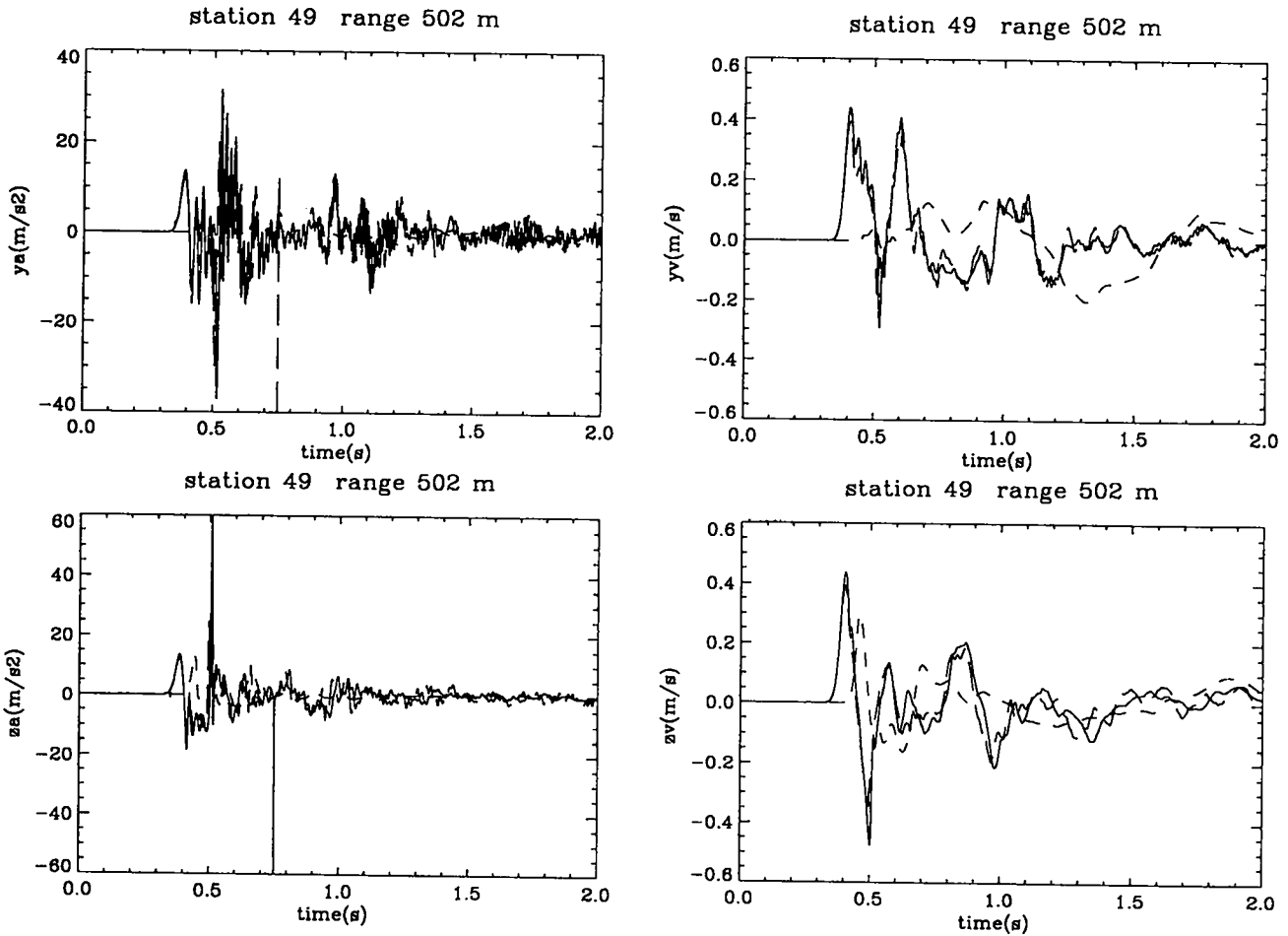
Figure 50: Experimental and computational free-surface results at 502 m. Shown are the radial acceleration ( m/s^2 ), radial velocity ( m/s ), vertical acceleration ( m/s^2 ), and vertical velocity ( m/s ) vs. time (s) at 502 m range from the NPE SGZ. The solid line denotes the CE simulation; the long dashed line represents the NE simulation; the short dashed line represents the NPE data collected by LANL [34], gage S11A.
