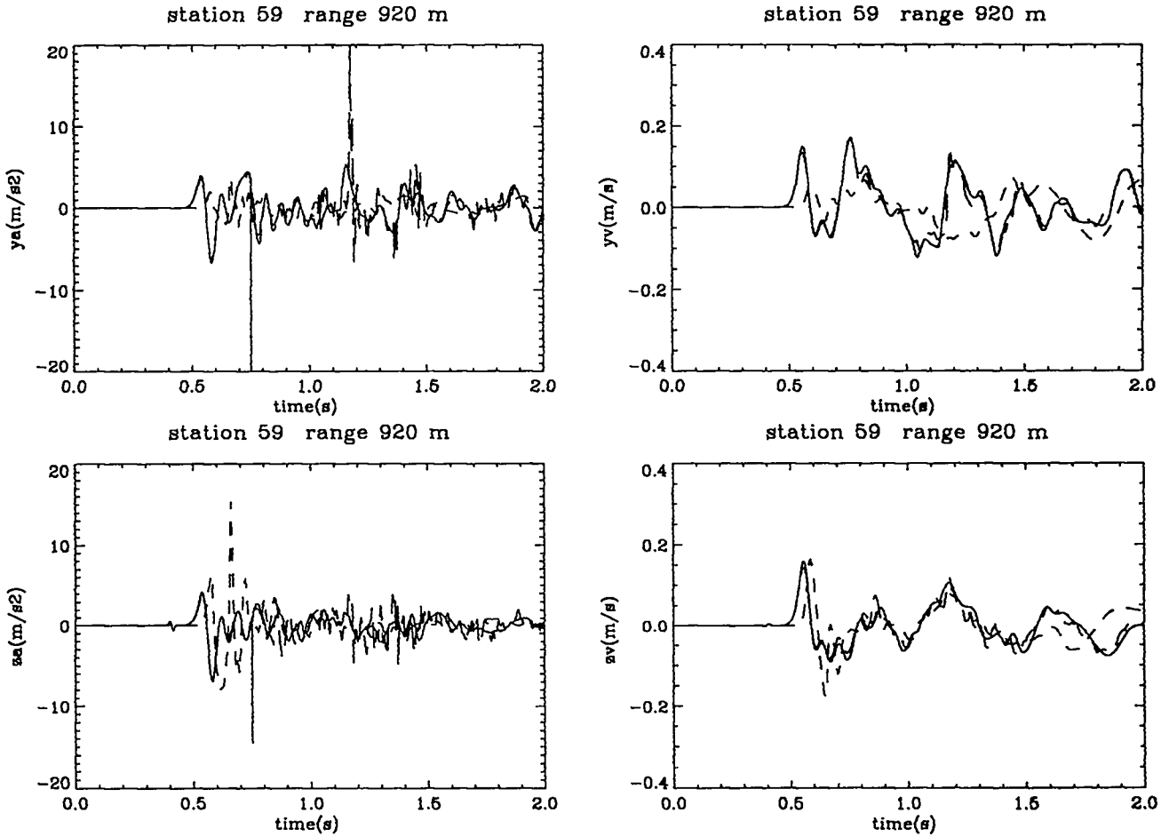
Figure 60: Experimental and computational free-surface results at 920 m. Shown are the radial acceleration (m/s 2 ), radial velocity (m/s), vertical acceleration (m/s 2 ), and vertical velocity (m/s) vs. time (s) at 920 m range from the NPE SGZ. The solid line denotes the CE simulation; the long dashed line represents the NE simulation; the short dashed line represents the NPE data collected by LANL [34], gage S12P.
