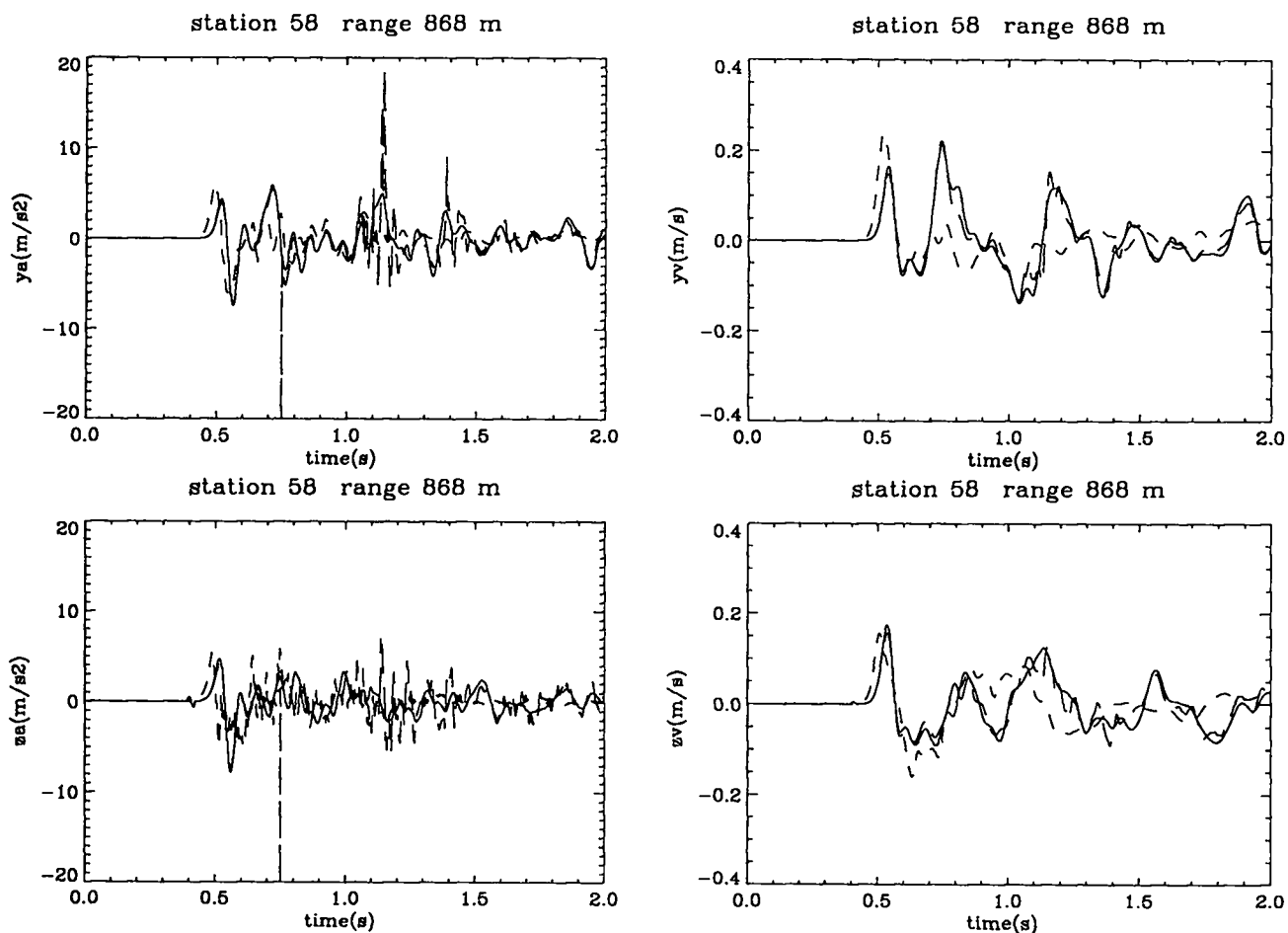
Figure 59: Experimental and computational free-surface results at 868 m. Shown are the radial acceleration (m/s 2 ), radial velocity (m/s), vertical acceleration (m/s 2 ), and vertical velocity (m/s) vs. time (s) at 868 m range from the NPE SGZ. The solid line denotes the CE simulation; the long dashed line represents the NE simulation; the short dashed line represents the NPE data collected by LANL [34], gage S4A.
