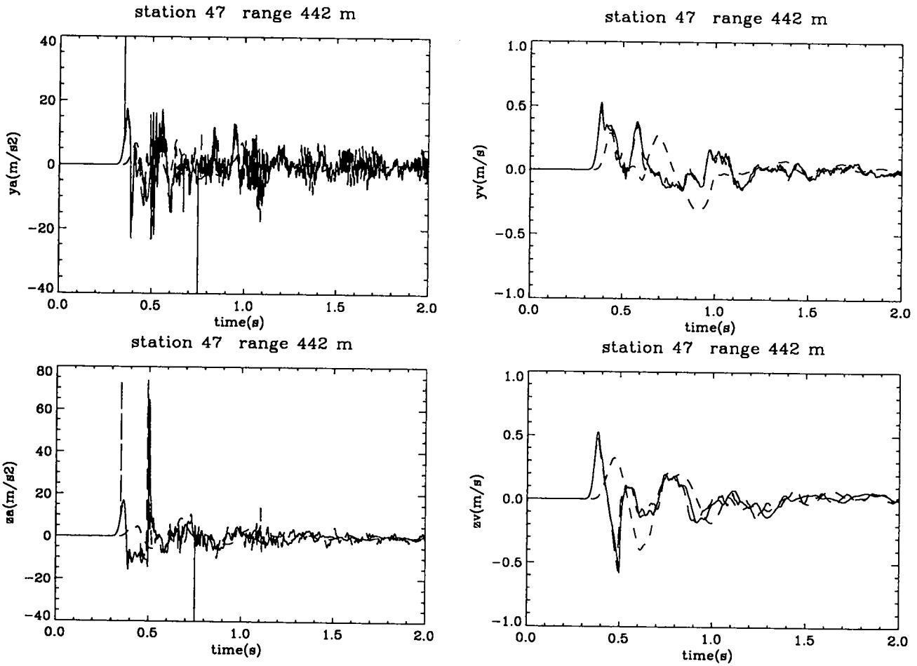
Figure 48: Experimental and computational free-surface results at 442 m. Shown are the radial acceleration ( m/s^2 ), radial velocity ( m/s ), vertical acceleration ( m/s^2 ), and vertical velocity ( m/s ) vs. time (s) at 442 m range from the NPE SGZ. The solid line denotes the CE simulation; the long dashed line represents the NE simulation; the short dashed line represents the NPE data collected by LLNL [33], gage S11P.
