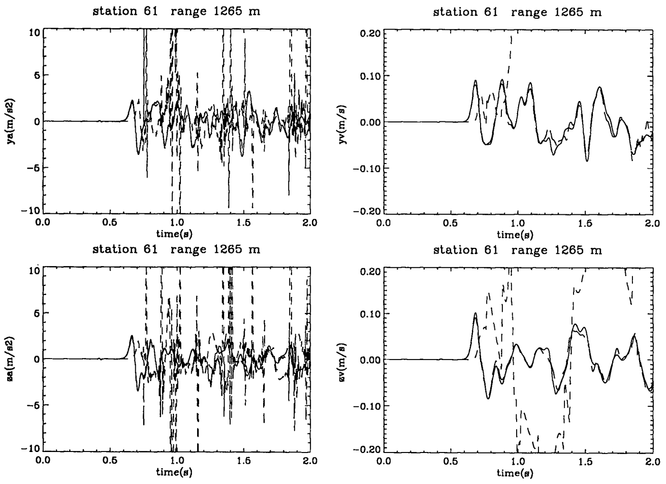
Figure 63: Experimental and computational free-surface results at 1265 m. Shown are the radial acceleration (m/s 2 ), radial velocity (m/s), vertical acceleration (m/s 2 ), and vertical velocity (m/s) vs. time (s) at 1265 m range from the NPE SGZ. The solid line denotes the CE simulation; the long dashed line represents the NE simulation; the short dashed line represents the NPE data collected by LANL [34], gage S2A. Although these gages obviously did not record the event correctly, we include this station for completeness.
